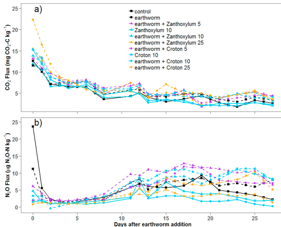
Fig. 3. (a) Times series of carbon dioxide ( \text{mg CO}_2\text{-C kg}^{-1} ) and (b) nitrous oxide ( \mu\text{g N}_2\text{O-N kg}^{-1} ) emission from soils with or without earthworms, and with or without two biochar types ( Croton megalocarpus and Zanthoxylum gillettii ) over 27 days of the experiment. Different line types represent presence/absence of earthworms, different symbols represent type of biochar, and different colors represent rate of biochar application.
