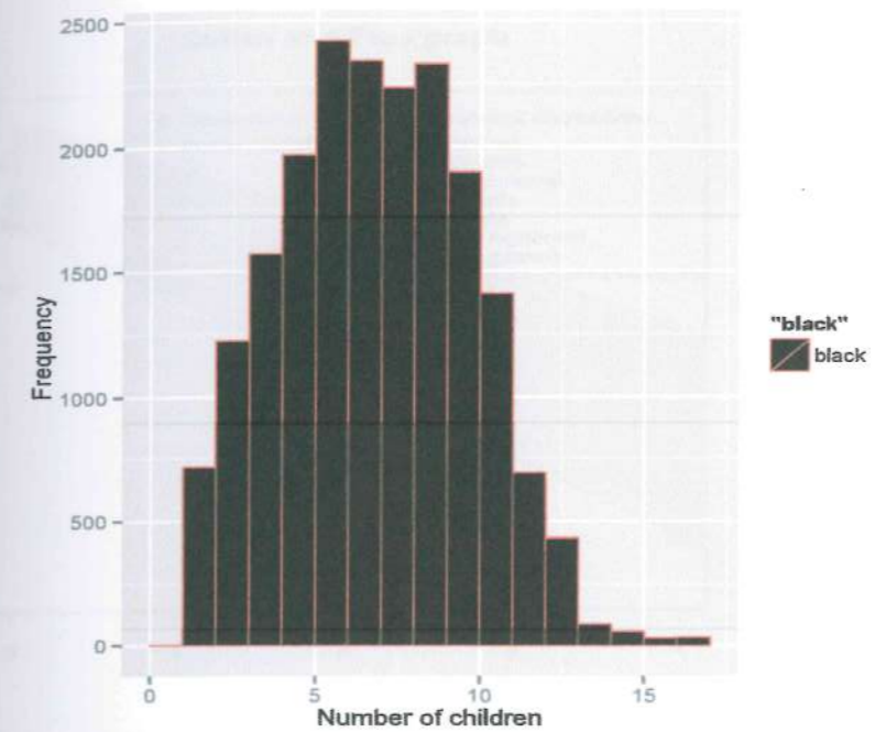
Figure 5.1: Histogram for Rwanda 2000 fertility data.
