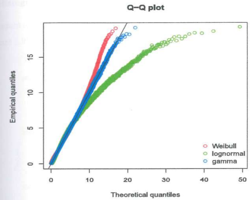
Figure 5.8: Q-Q plots for Gamma, Weibull and Lognormal for Indonesia 2007 fertility data.
