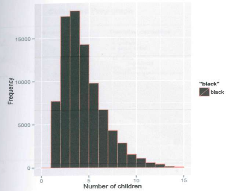
Figure 5.5: Histogram for Indonesia 2007 fertility data
