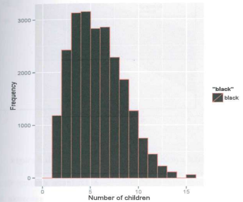
Figure 5.9: Histogram for Kenya 2009 fertility data.
