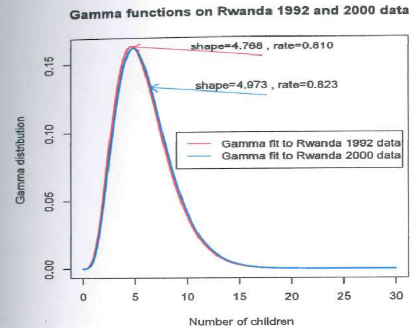
Figure 6.1: Gamma fit on Rwanda 1992 and on Rwanda 2000 data on the same scale
