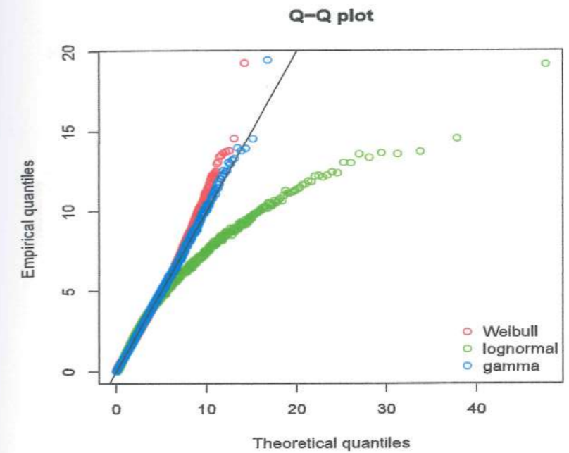
Figure 4.8: Q-Q plots for Gamma, Weibull and Lognormal for Indonesia 2002 fertility data.
